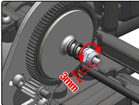
Tighten or loosen the nut to have 3mm of visible shaft.
