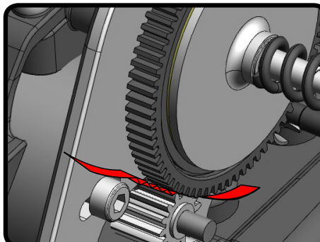
Cut a 5mm wide strip of paper and run it between the pinion and the spur gear.
